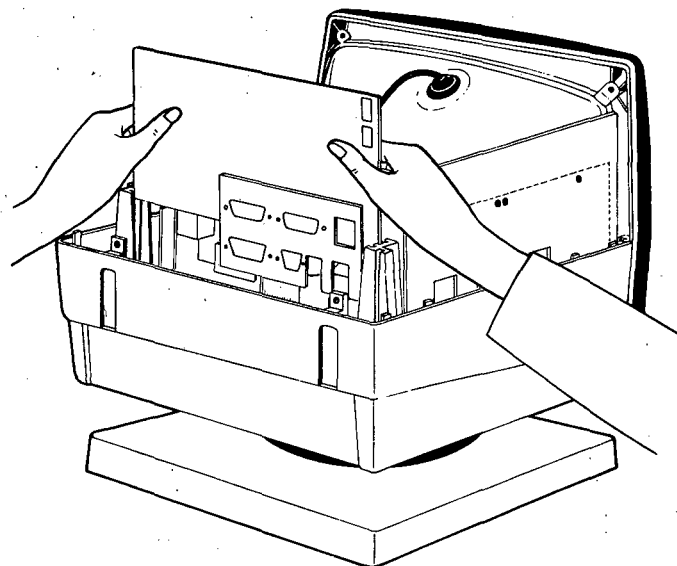
Figure 1-15 Removing the Logic Board and Shroud from the Card Guide
