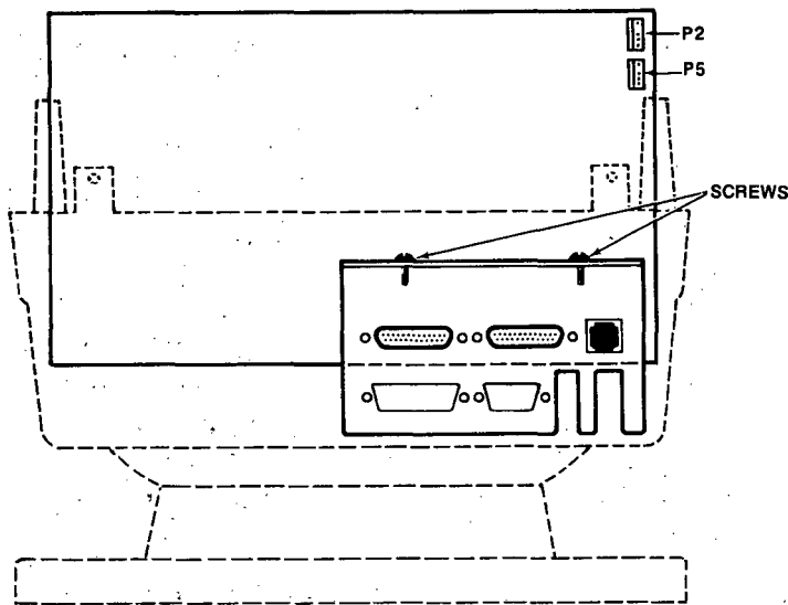
Figure 1-14 Connectors P2 and P5 on Logic Board
