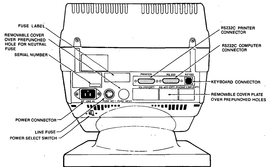
Figure 1-10 Rear View of Terminal
